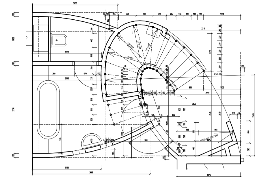
PÔDORYS - DETAIL
