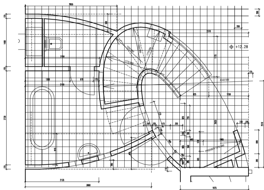
PÔDORYS - DETAIL
