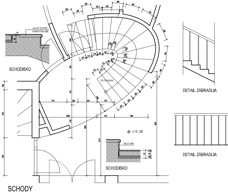
PÔDORYS - DETAIL
